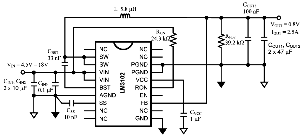
Typical Application Schematic for V_{OUT} = 0.8V
