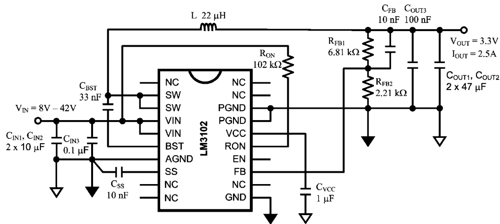
Typical Application Schematic for V_{OUT} = 3.3V
