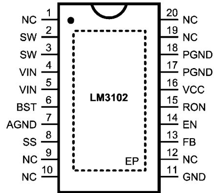
30021302 20-lead Plastic eTSSOP NS Package Number MXA20A
