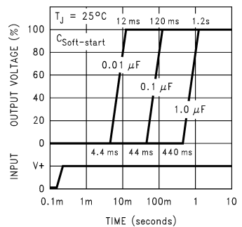
Soft-start Response
