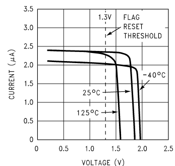
Delay Pin Current
