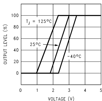
Soft-start
