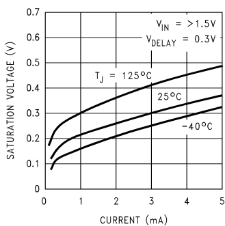
Flag Saturation Voltage
