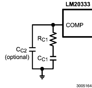
FIGURE 4. Compensation Network for LM20333
