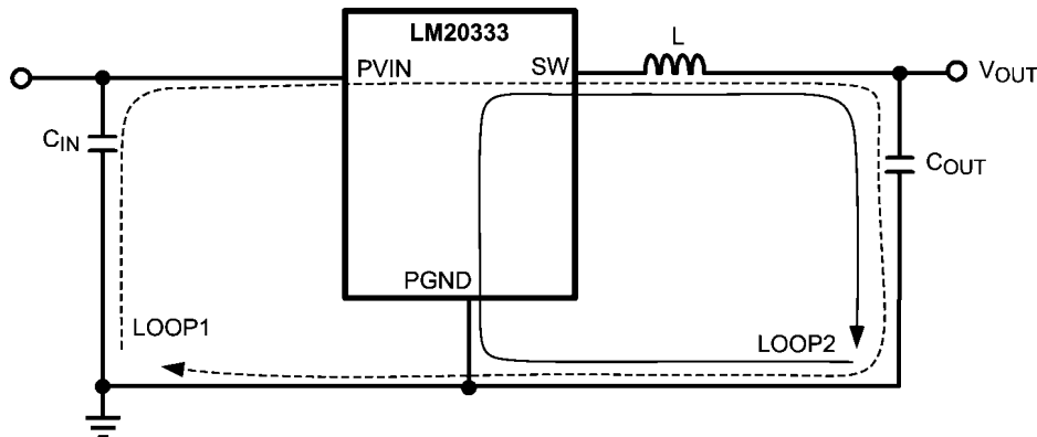
FIGURE 13. Schematic of LM20333 Highlighting Layout Sensitive Nodes
