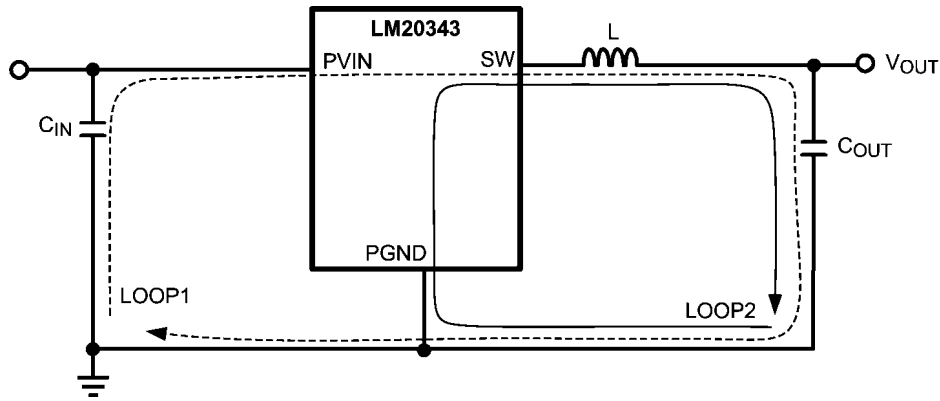
FIGURE 13. Schematic of LM20343 Highlighting Layout Sensitive Nodes
