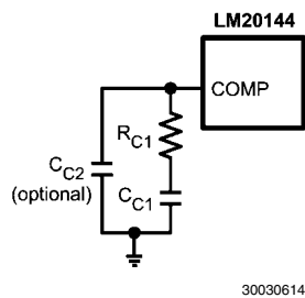
FIGURE 5. Compensation Network for LM20144
