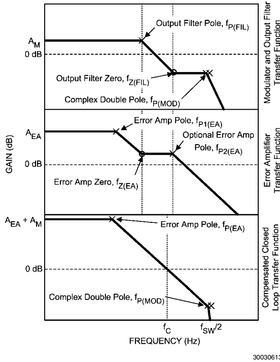
FIGURE 4. LM20144 Loop Compensation
