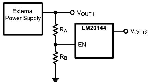
FIGURE 6. Sequencing LM20144 with Precision Enable
