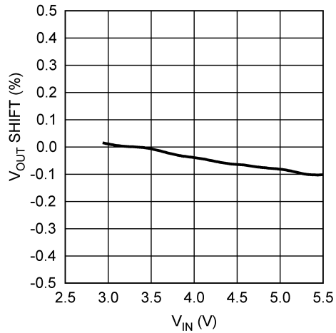
Line Regulation
