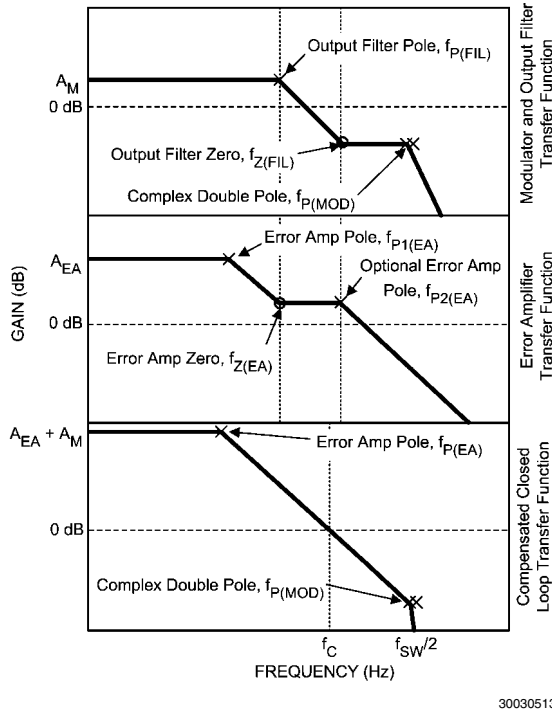
FIGURE 4. LM20143 Loop Compensation
