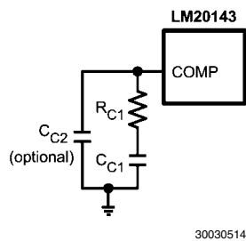
FIGURE 5. Compensation Network for LM20143
