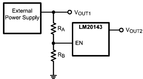
FIGURE 6. Sequencing LM20143 with Precision Enable
