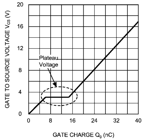
FIGURE 4. Typical MOSFET Gate Charge Curve
