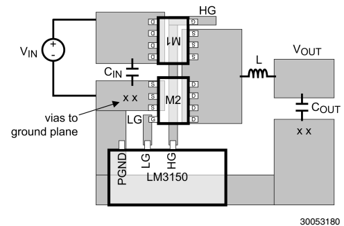
FIGURE 7. PCB Placement of Power Stage
