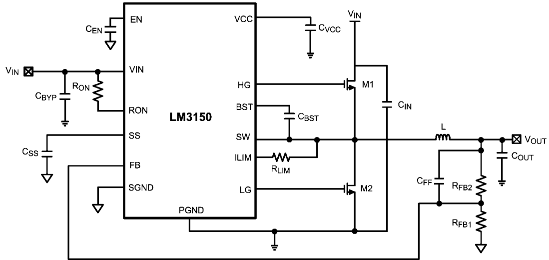
FIGURE 5. Design Example Schematic
