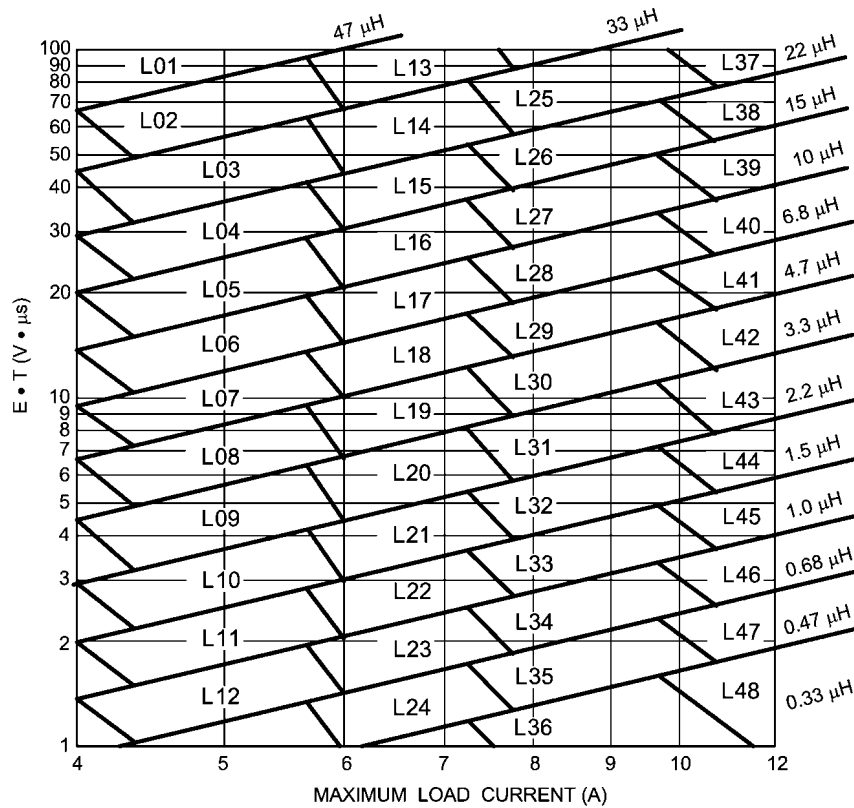
FIGURE 3. Inductor Nomograph
