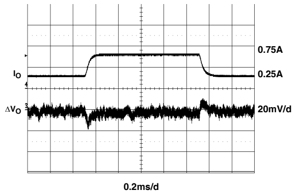
FIGURE 10. TRANSIENT RESPONSE
