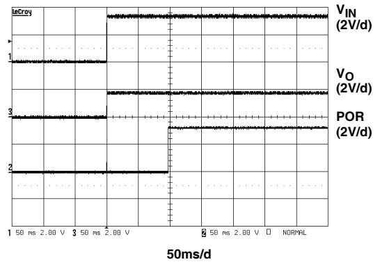
FIGURE 8. START-UP 2
