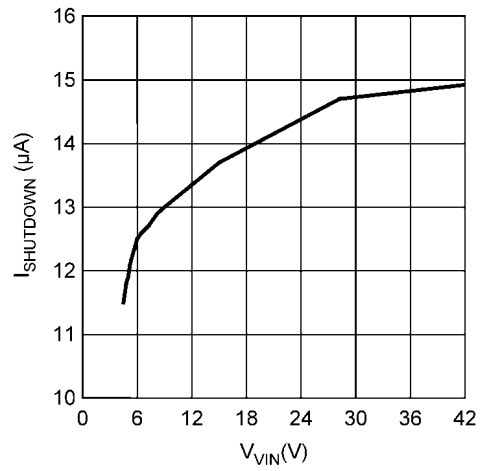
Shutdown Current
