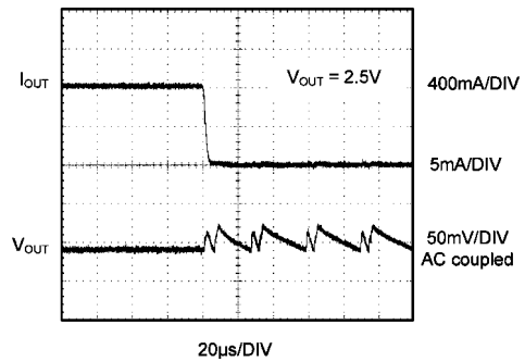
Load Transient Reponse ( V_{OUT} = 2.5V , ECO Mode to PWM Mode)
