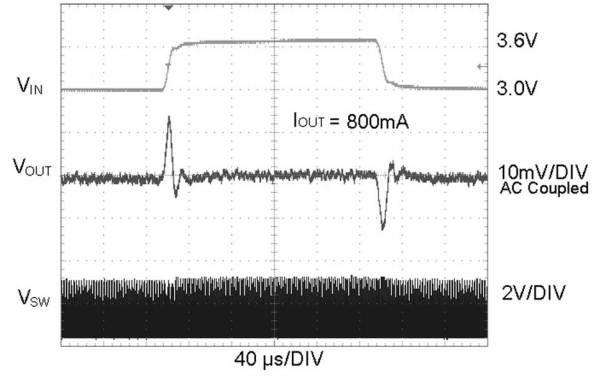
Line Transient Reponse ( V_{OUT} = 0.75V , PWM Mode)
