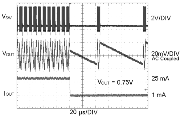
Load Transient Reponse ( V_{OUT} = 0.75V , ECO Mode 25 mA to 1mA)
