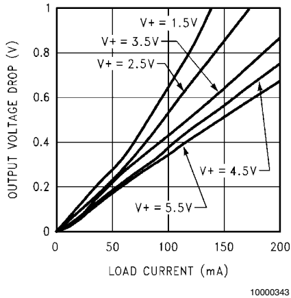
Output Voltage Drop vs Load Current
