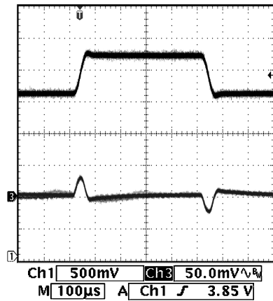
Line Transient (LDO1) 3.6 - 4.2\text{V}_{IN} , 2.6\text{V}_{OUT} , 300mA load
