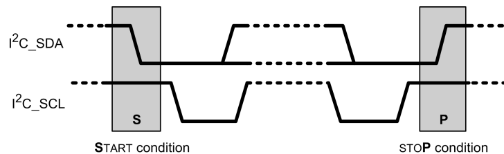
START and STOP Conditions
