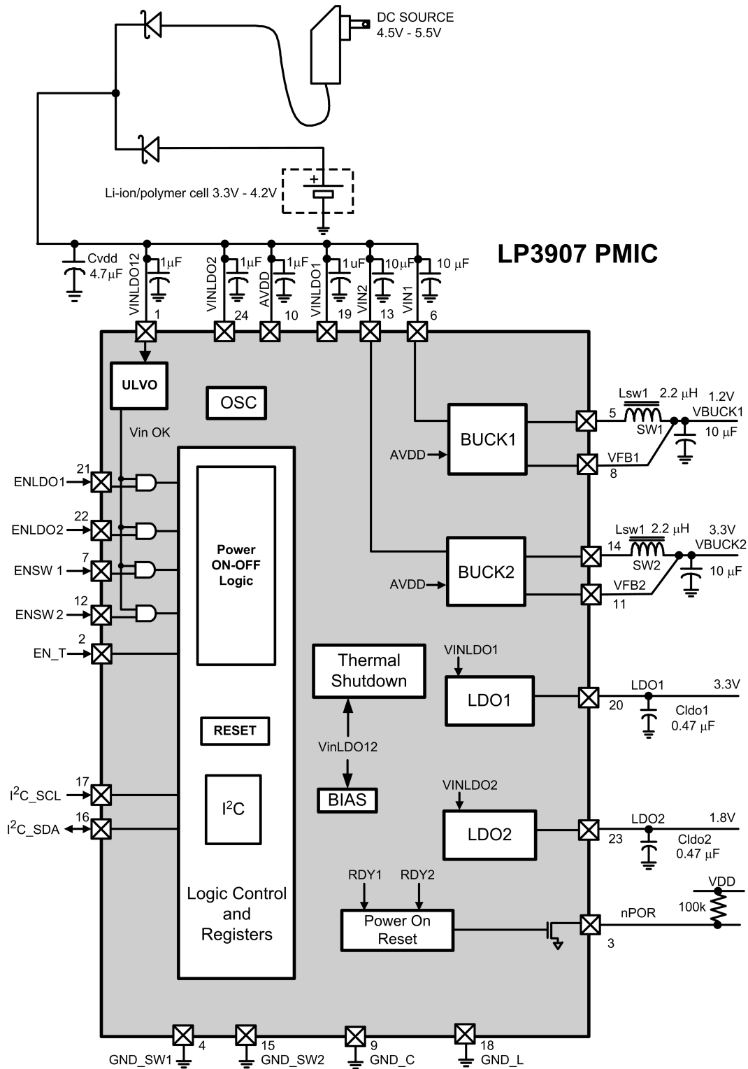
FIGURE 2. Application Circuit
