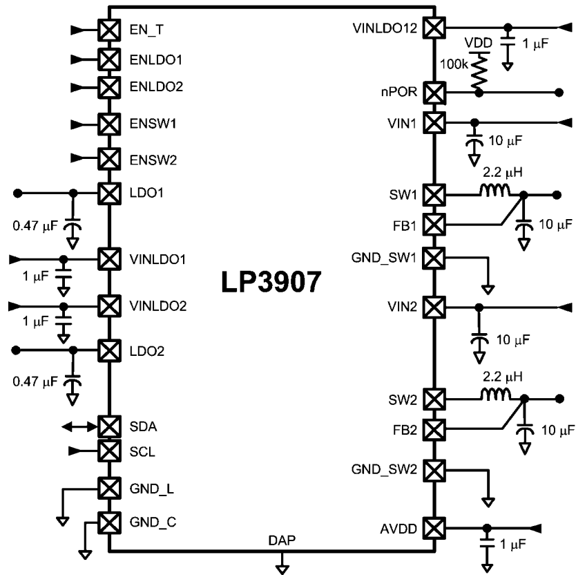
FIGURE 1. Application Circuit
