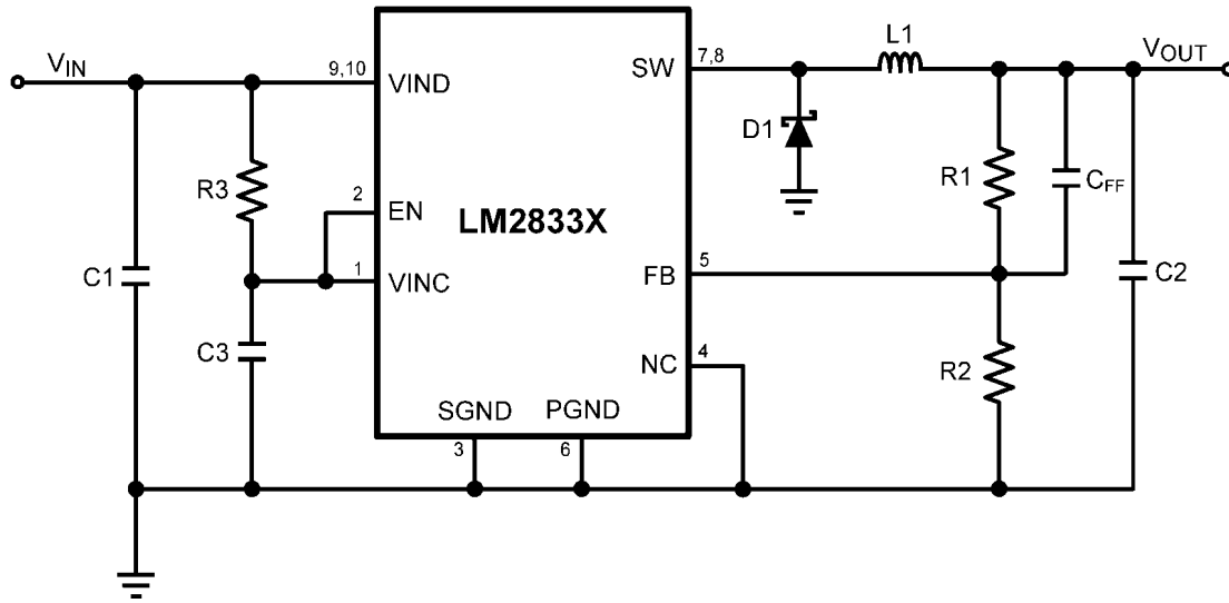
FIGURE 12. LM2833X (1.5MHz): V_{IN} = 5V , Output = 3.3V/3.0A
