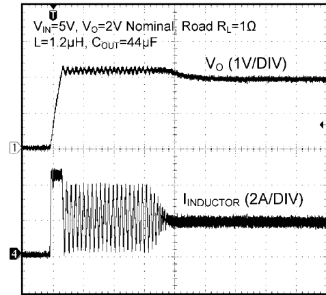
Recovery from Thermal Shutdown - "LM2833X"
