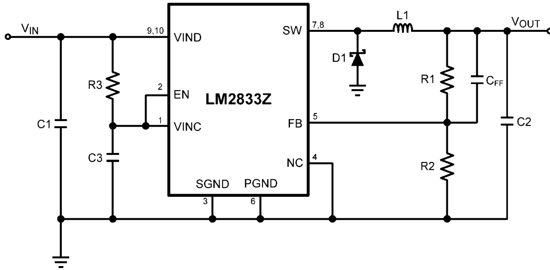
FIGURE 14. LM2833Z (3MHz): V_{IN} = 5V , Output = 3.3V/3.0A
