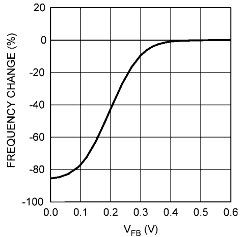
Frequency Foldback
