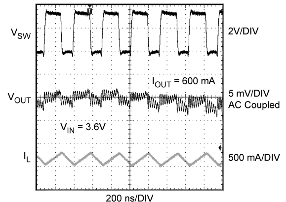
FIGURE 6. Typical PWM Operation
