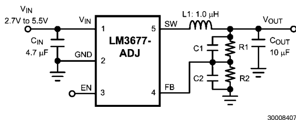
FIGURE 2. Typical Application Circuit - ADJ. Version
