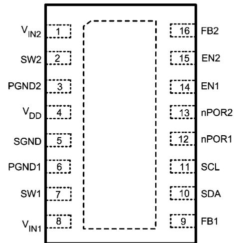
FIGURE 4. Top View
