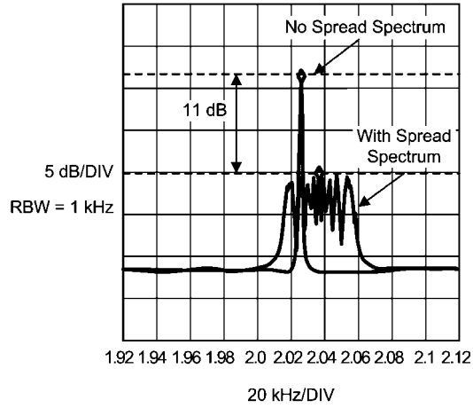
Spread Spectrum Enabling ( V_{OUT} Signal at 2 MHz)
