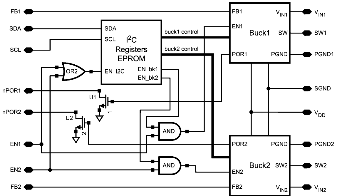
FIGURE 2. Functional Diagram
