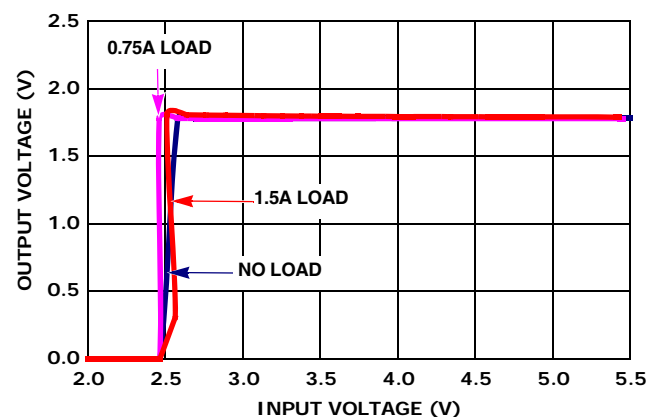
FIGURE 12. OUTPUT VOLTAGE REGULATION vs V_{IN} PWM MODE
