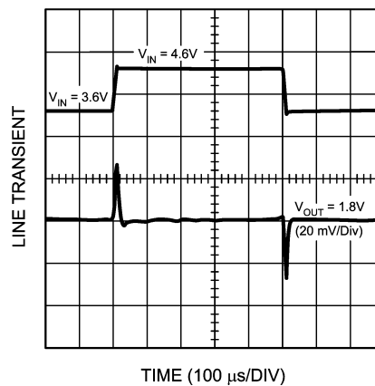
Line Transient ( V_{IN} = 3.6V to 4.6V , I_{LOAD} = 100\text{ mA} )
