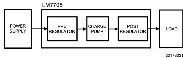
FIGURE 2. LM7705 Architecture
