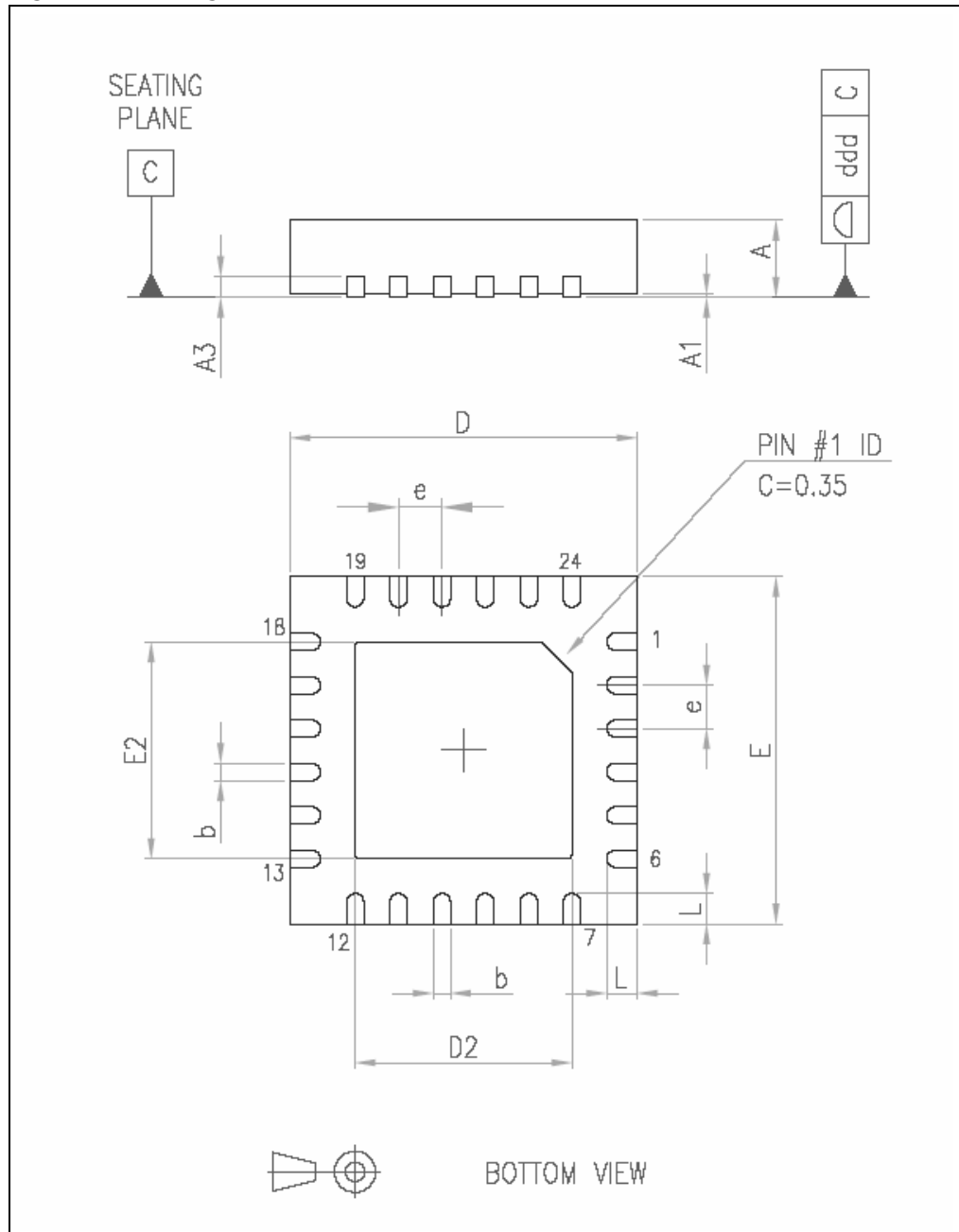
Figure 41. Package dimensions
