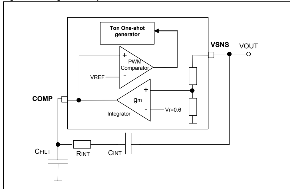
Figure 39. Integrative compensation
