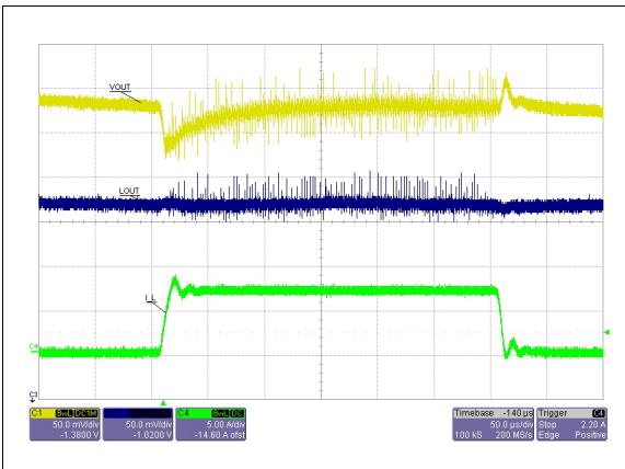
Figure 14. V_{OUT} Load Transient ( V_{IN} = 24V , LOAD = 0A \rightarrow 7A @2.5A/\mu s ), pulse-skip mode
