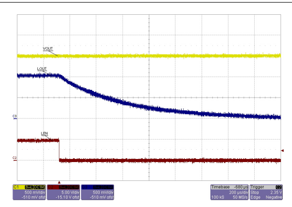
Figure 19. OV protection, pulse-skip mode
