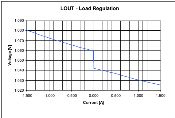
Figure 8. L_{OUT} load regulation L_{DOIN} = V_{OUT} , V_{OUT} in forced PWM mode
