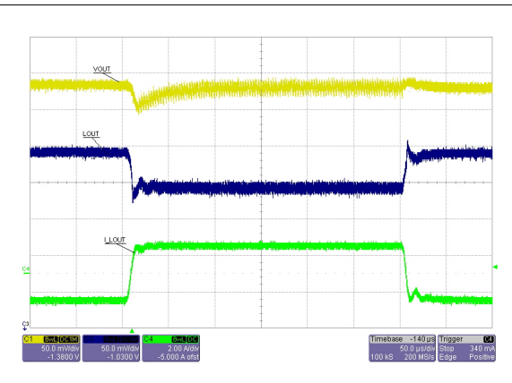
Figure 15. V_{OUT} load transient ( V_{IN} = 24V , LOAD = -1.5A \rightarrow 1.5A @2.5A/\mu s ), pulse-skip mode
