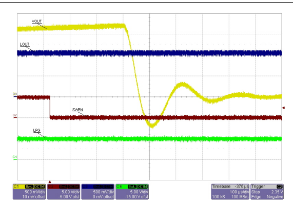
Figure 21. LOUT current limit during an output short
