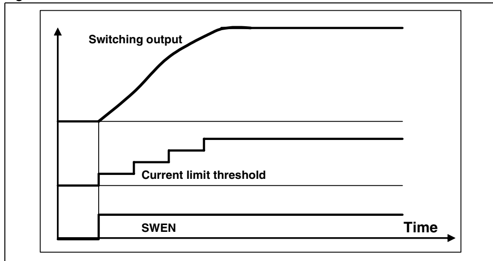
Figure 31. Soft-start waveforms
