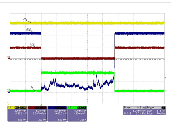
Figure 21. LOUT current limit during an output short
