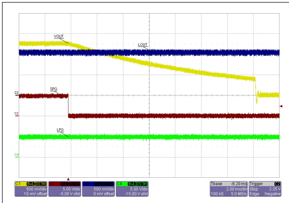
Figure 20. VOUT current limit protection during a load transient (0 A to 9 A @2.5A/μs)
