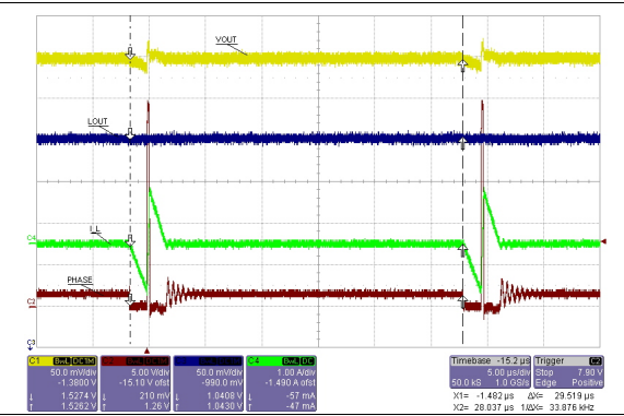
Figure 13. LOUT turn on, V_{OUT} in pulse-skip mode
