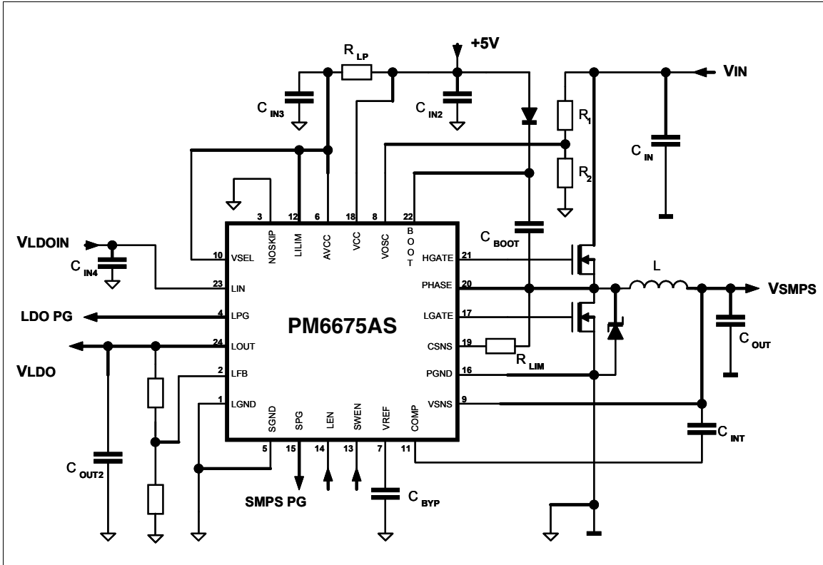
Figure 1. Application circuit
