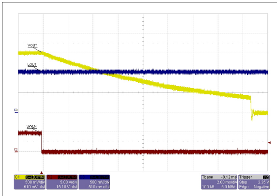
Figure 18. UV protection, pulse-skip mode LOUT powered by an auxiliary rail
