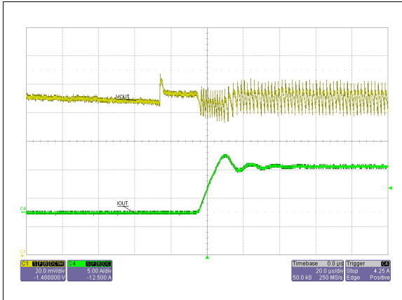
Figure 27. 0 A to 5 A VOUT load transient, Pulse-Skip
