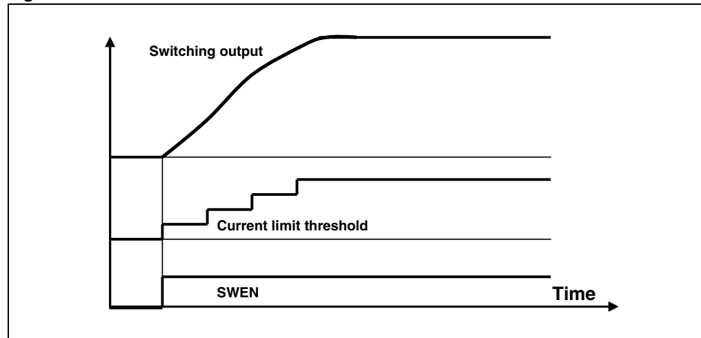
Figure 41. Soft-start waveforms
