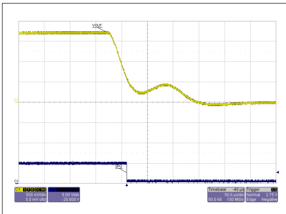
Figure 29. Over-voltage protection, VOUT = 1.5 V
