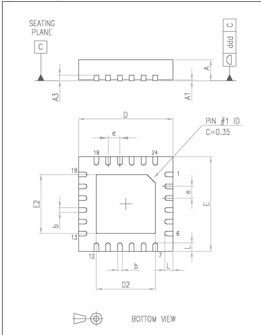
Figure 51. Package dimensions
