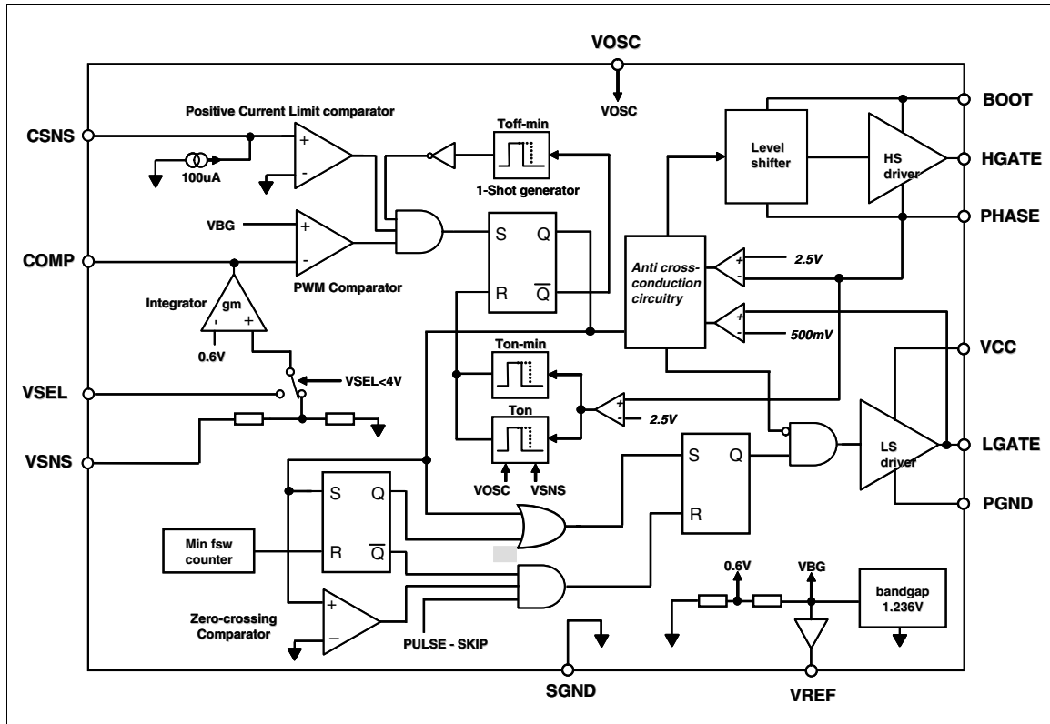
Figure 34. Switching section simplified block diagram
