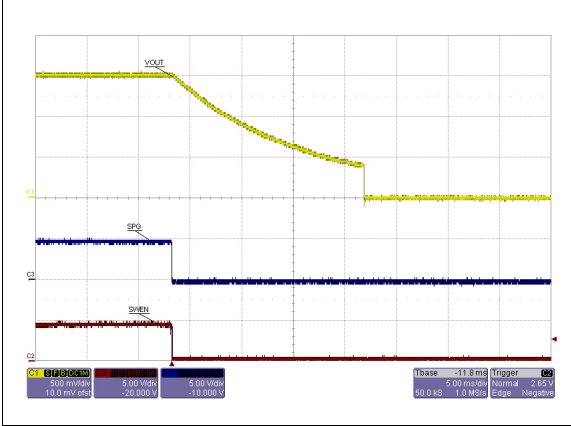
Figure 21. Switching section output soft-end
