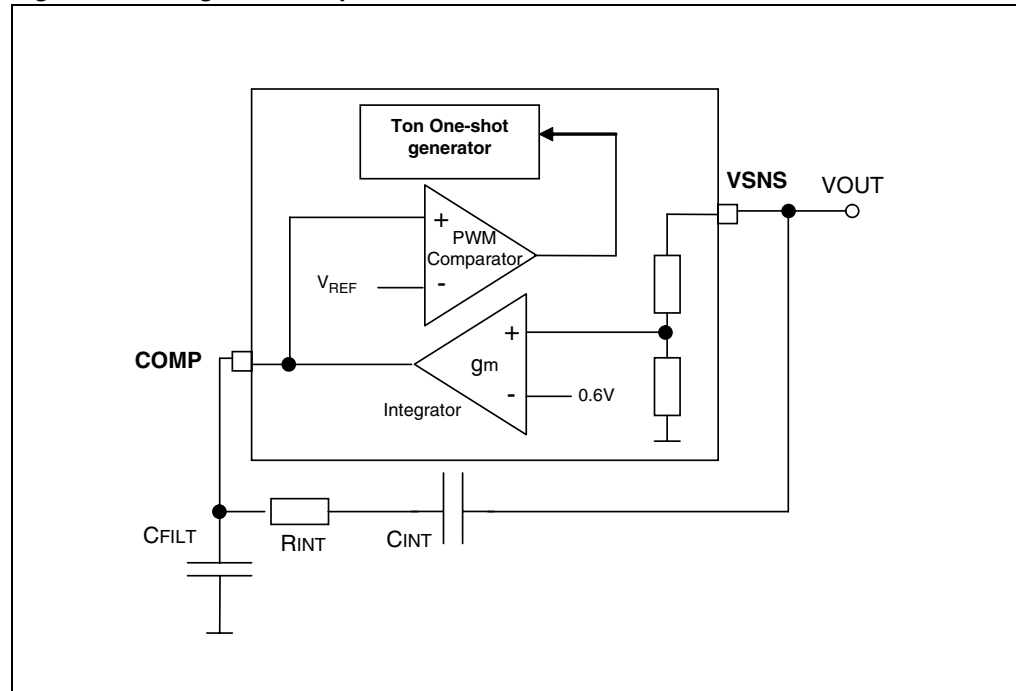
Figure 49. Integrative compensation
