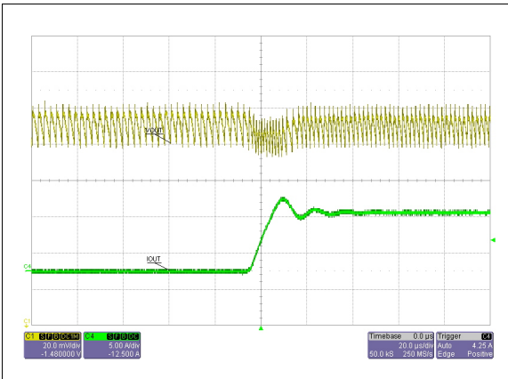
Figure 25. 0 A to 8 A VOUT load transient, PWM
