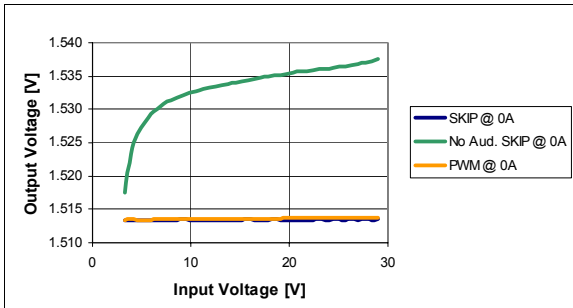
Figure 9. VOUT line regulation, 1.5 V, 0 A
