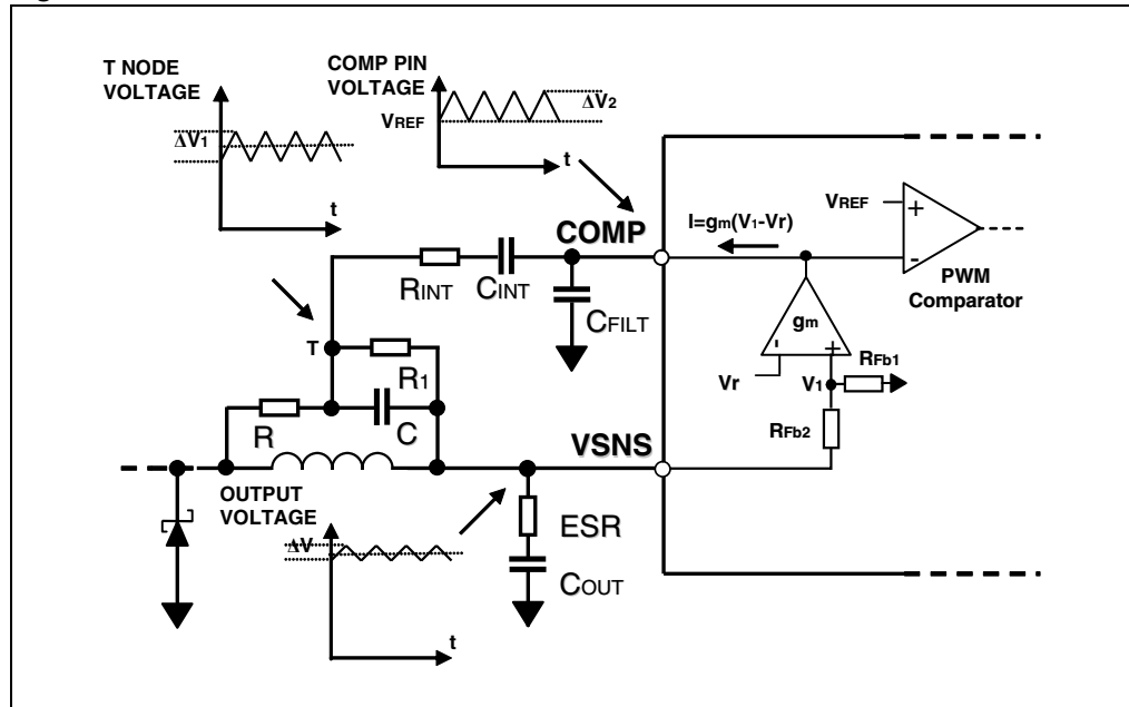
Figure 36. "Virtual-ESR" network
