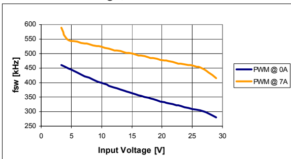
Figure 13. Switching frequency vs input voltage, 1.5 V
