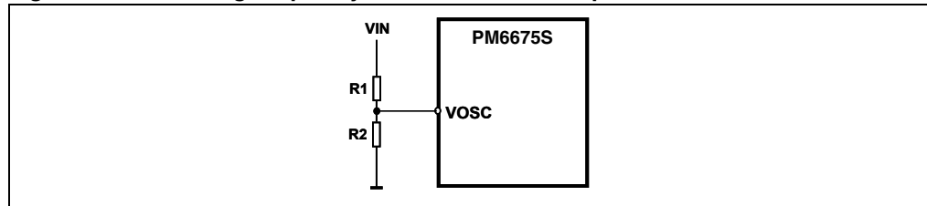
Figure 33. Switching frequency selection and VOSC pin
