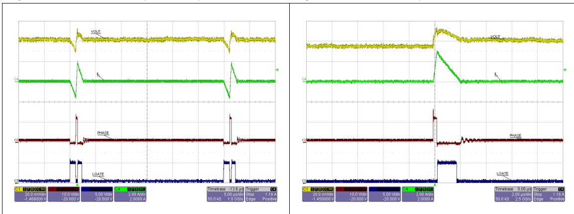
Figure 17. No-audible pulse-skip waveforms Figure 18. Pulse-skip waveforms
