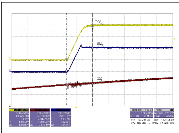
Figure 19. Power-up sequence VCC above UVLO
