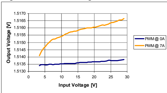
Figure 11. VOUT line regulation, 1.5 V
