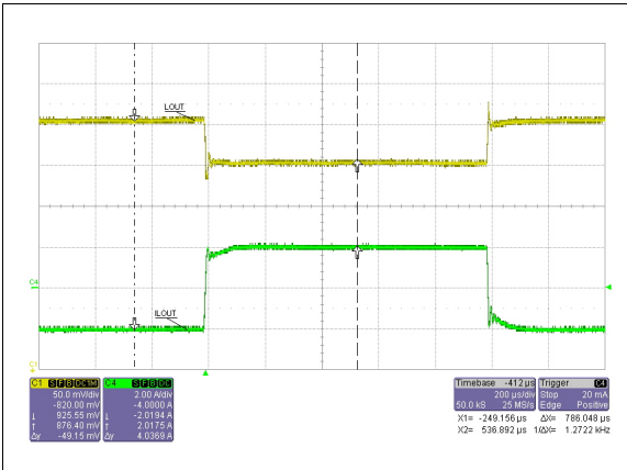
Figure 23. -1.8 A to 1.8 A LOUT load transient, 0.9 V
