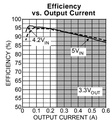
Figure 2. Efficiency Curve
