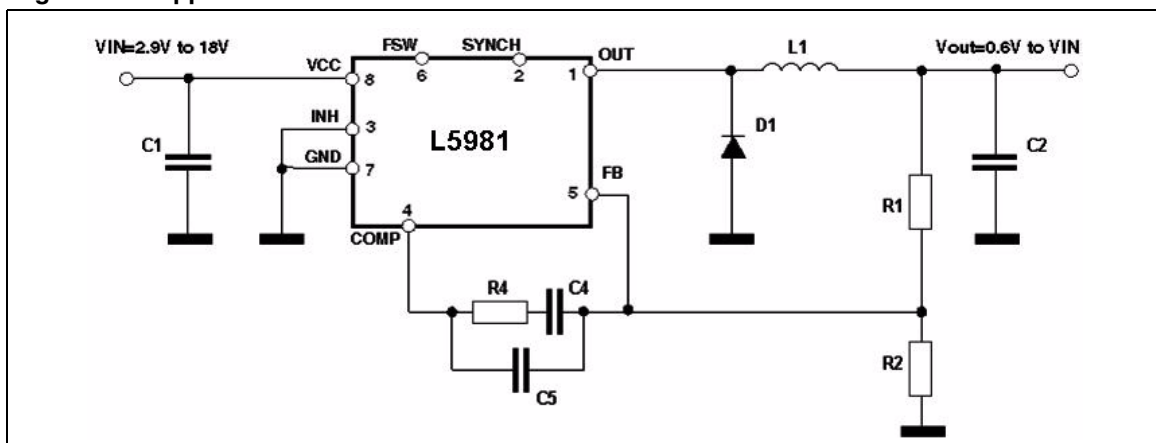
Figure 1. Application circuit
