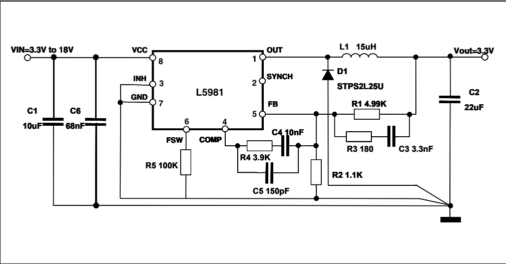
Figure 18. Demonstration board application circuit
