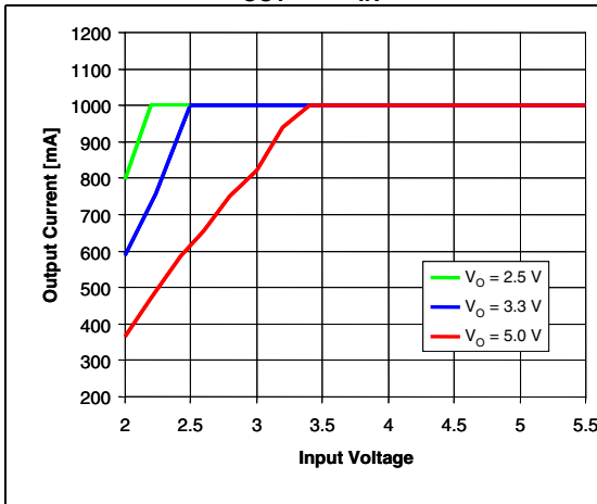
Figure 9. Max I_{O\text{UT}} vs. V_{IN}
