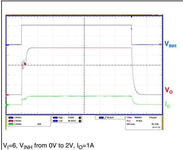
Figure 30. INH transient
