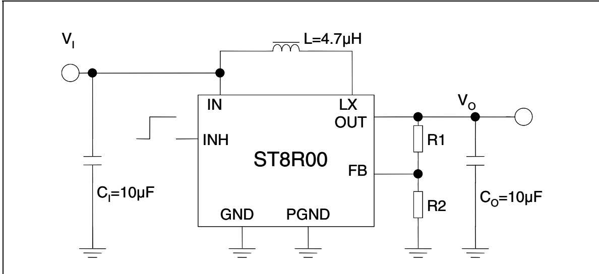
Figure 3. Application circuit
