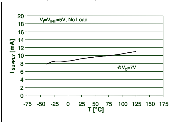
Figure 8. Supply current vs temperature (for ST8R00W)
