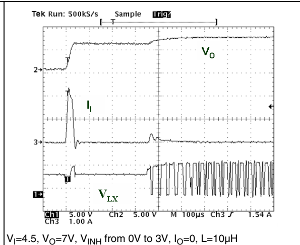
Figure 31. Inrush current
