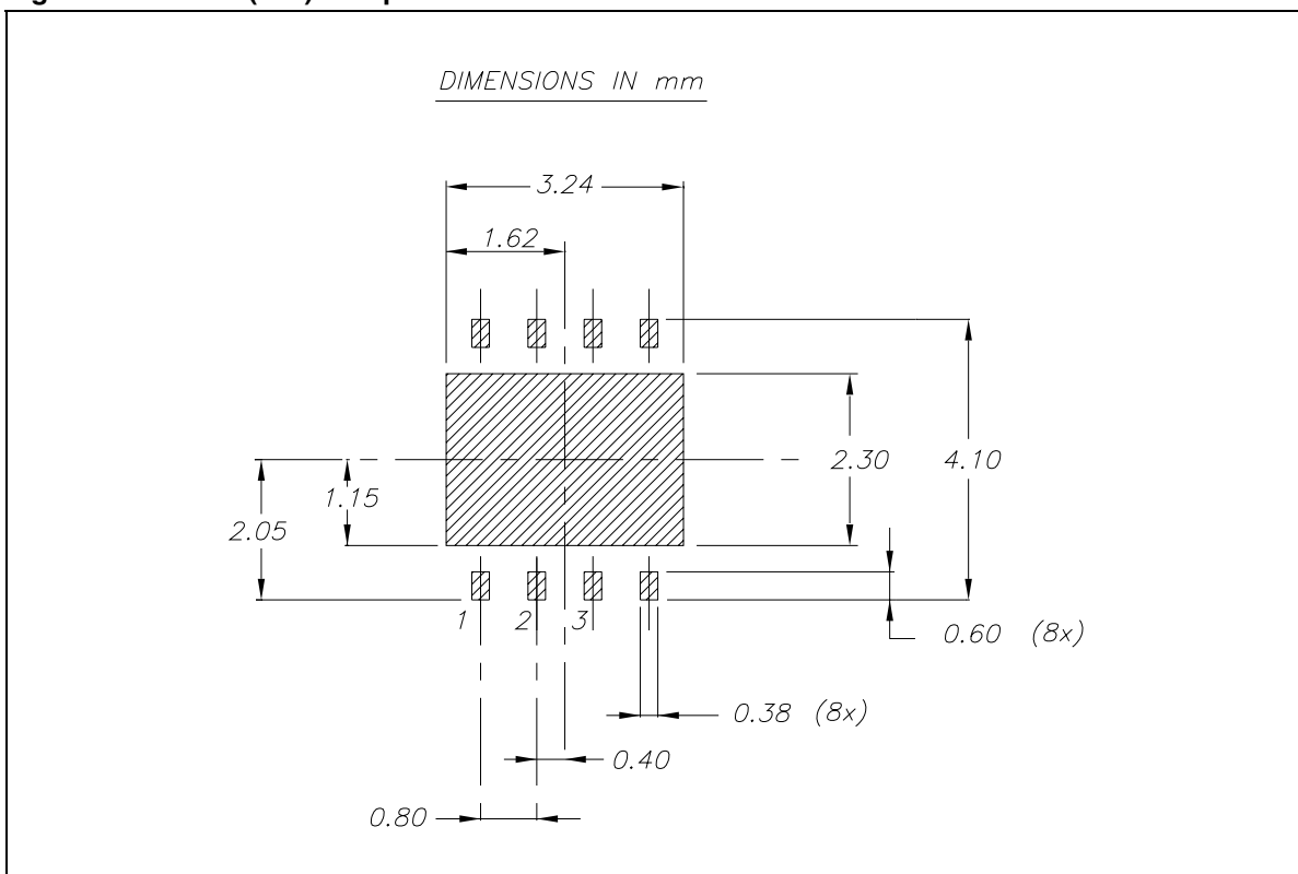
Figure 32. DFN8 (4x4) Footprint Recommended Data
