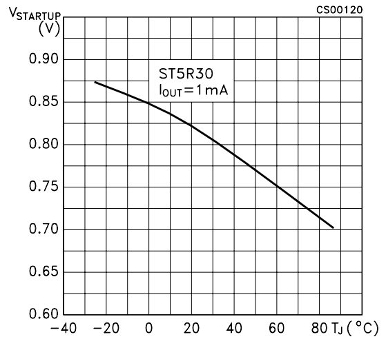
Figure 21: Start-up Voltage (V IN - V F ) vs Temperature
