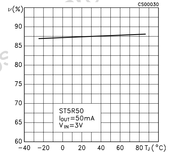
Figure 11: Efficiency vs Temperature
