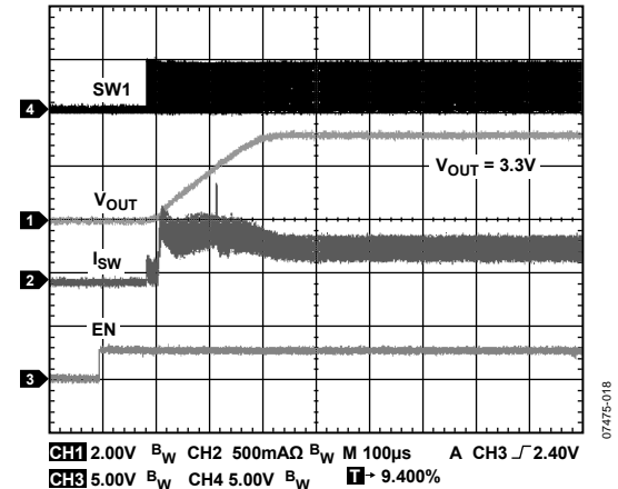
Figure 26. Startup into PWM Mode (V OUT = 3.3 V, I OUT = 300 mA)
