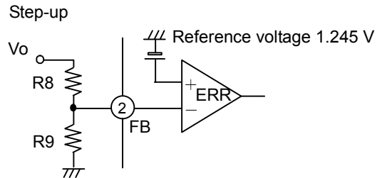
Fig. 25 Feedback Resistor Setting
