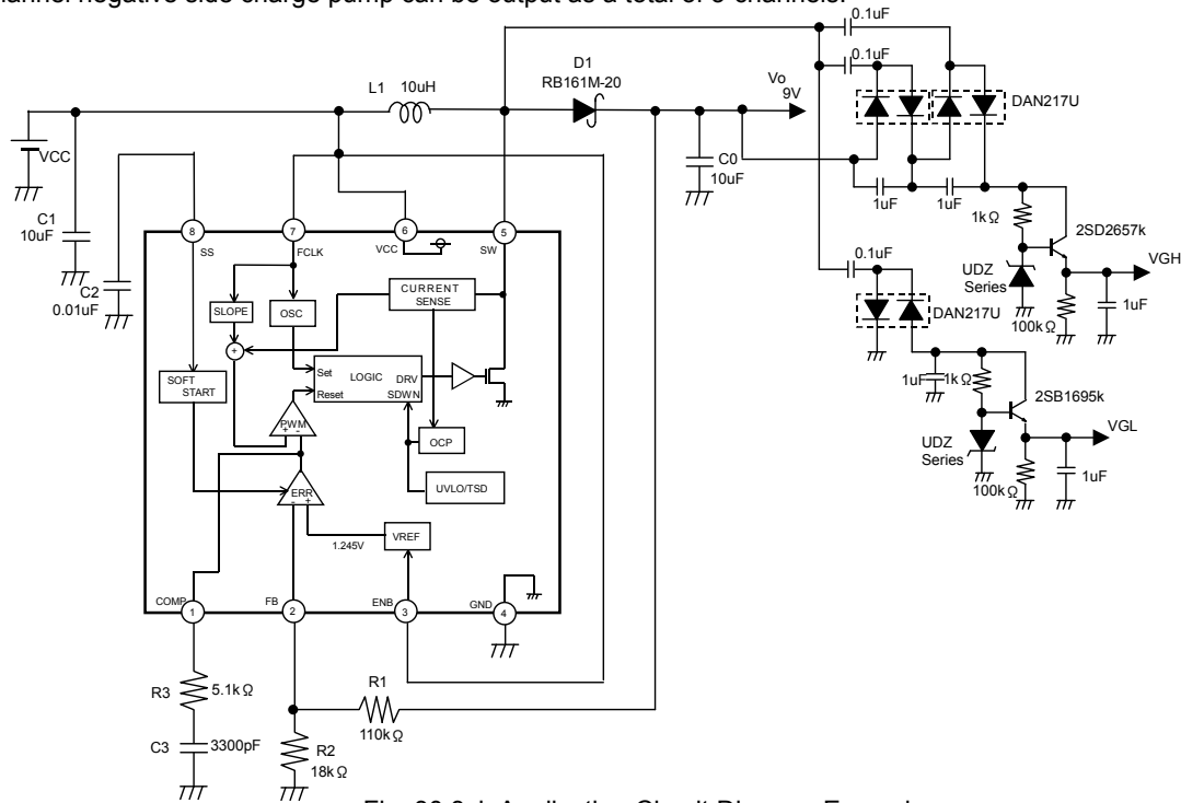
Fig. 30 3ch Application Circuit Diagram Example
