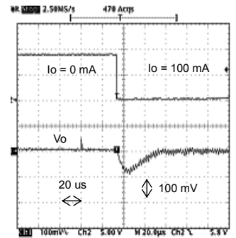
Fig. 15 Load Response Waveform
