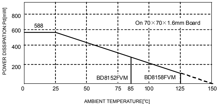
Fig. 37 Power Dissipation Reduction
