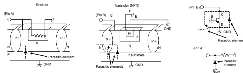
Fig.36 Example of a Simple Monolithic IC
