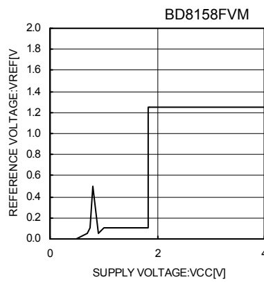
Fig. 5 Reference Voltage vs Power Supply Voltage
