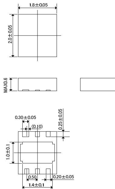
USP-6C Package
