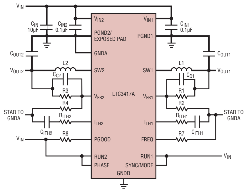
Figure 5. Layout Guideline
