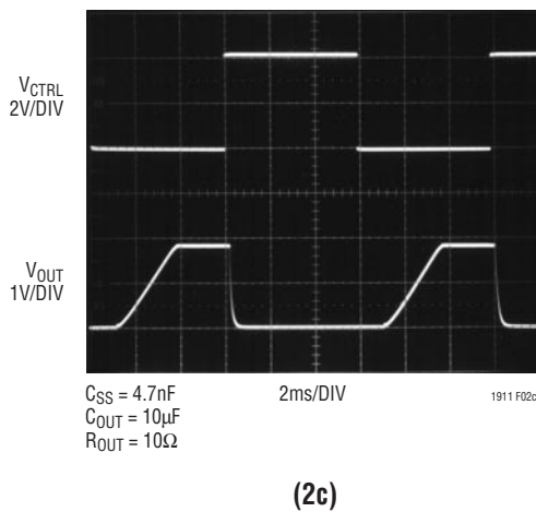
Figure 2. Shutdown/Soft-Start Operation
