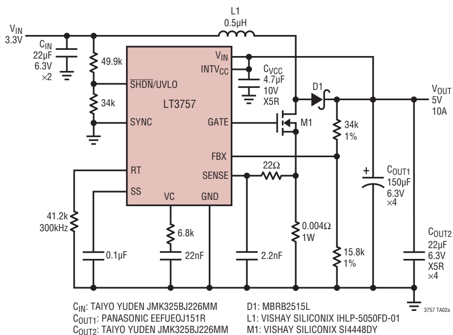
3.3V Input, 5V/10A Output Boost Converter
