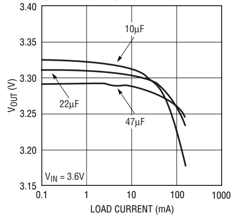
Load Regulation vs C_{OUT} (3.3V Version)
