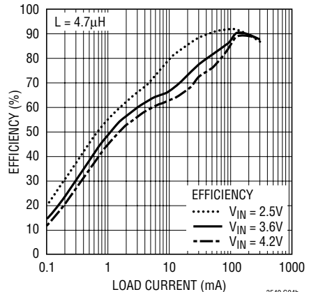
Efficiency vs Load Current, V_{OUT} = 1.8V , Pulse Skip
