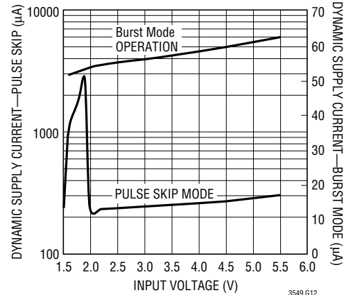
Dynamic Input Current VOUT = 1.5V, 247kΩ Load
