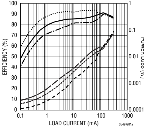
Efficiency/Power Loss vs Load Current, V_{OUT} = 1.5V , Burst Mode
