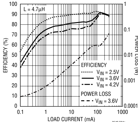
Efficiency vs Load Current, V_{OUT} = 1.8V , Burst Mode
