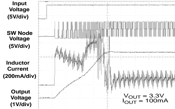
Start-up Response
