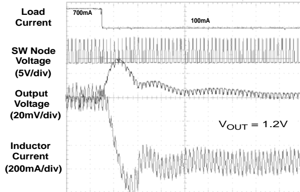
Transient Response
