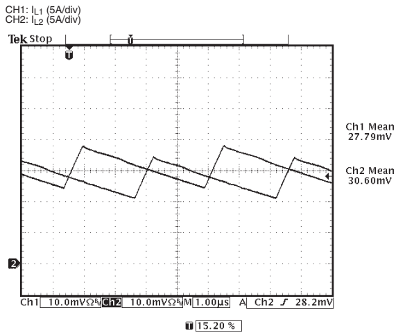
CURRENT SHARING, 30A LOAD
