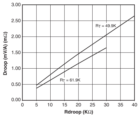
DROOP VS. R DROOP
