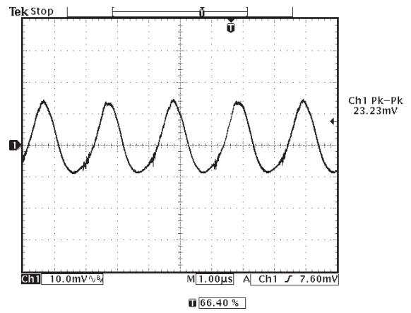
OUTPUT RIPPLE, 70A LOAD
