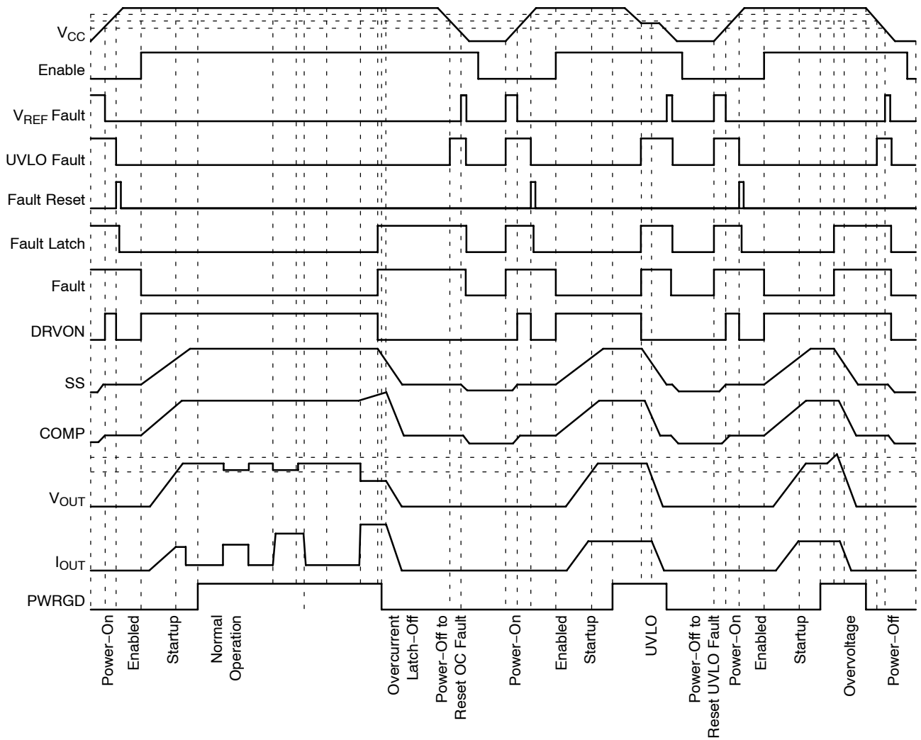
Figure 16. Operating Waveforms
