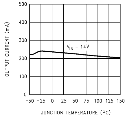
Peak Output Current ( V_{buf} )
