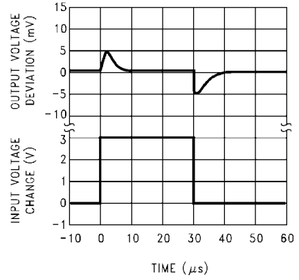
Line Transient Response ( V_{buf} )
