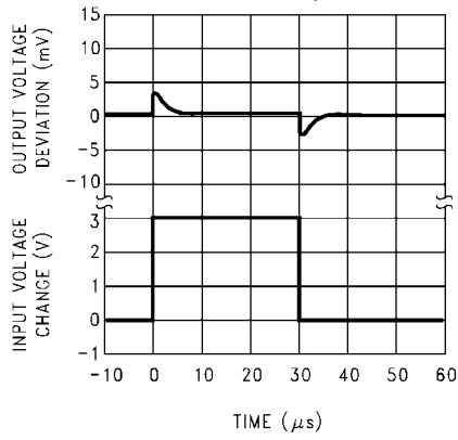
Line Transient Response ( V_{stby} )
