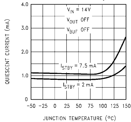
Quiescent Current ( V_{stby} )
