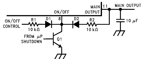
FIGURE 1. Power Down Override
