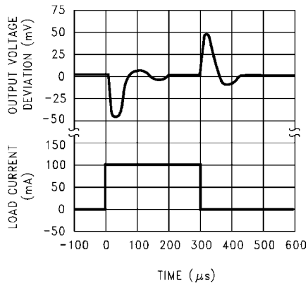
Load Transient Response ( V_{buf} )
