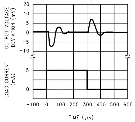
Load Transient Response ( V_{stby} )
