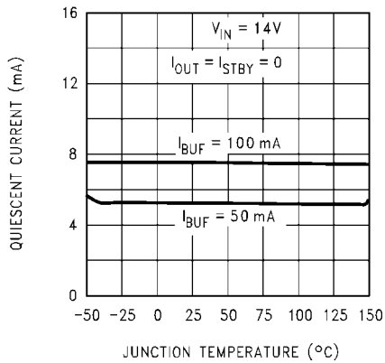
Quiescent Current ( V_{buf} )
