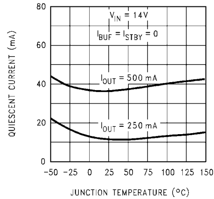
Quiescent Current ( V_{OUT} )
