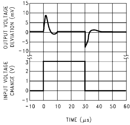
Line Transient Response ( V_{OUT} )
