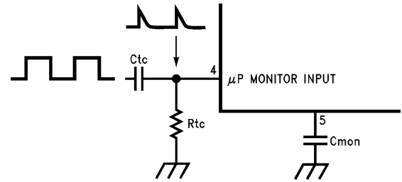
FIGURE 2. Monitoring Square Wave \mu\text{P} Signals
