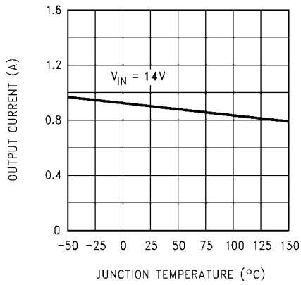
Peak Output Current ( V_{OUT} )
