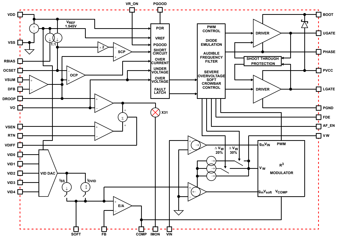
FIGURE 1. SIMPLIFIED FUNCTIONAL BLOCK DIAGRAM OF THE ISL6263B
