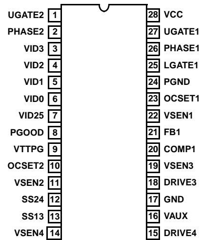
ISL6523 (SOIC) TOP VIEW
