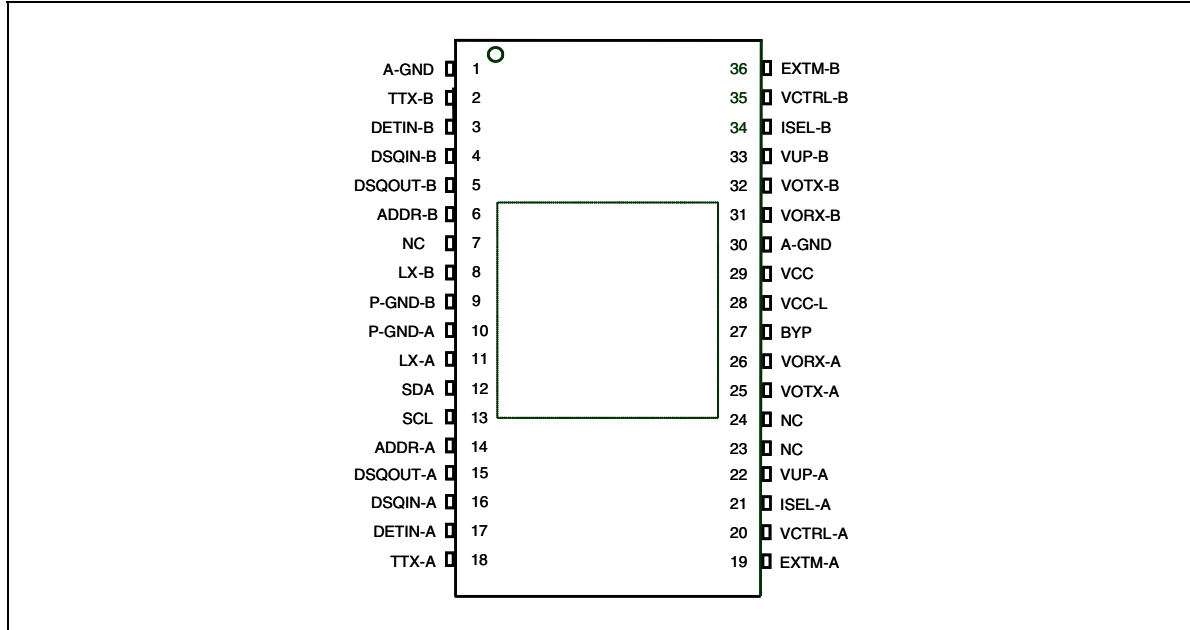
Figure 3. Pin connections
