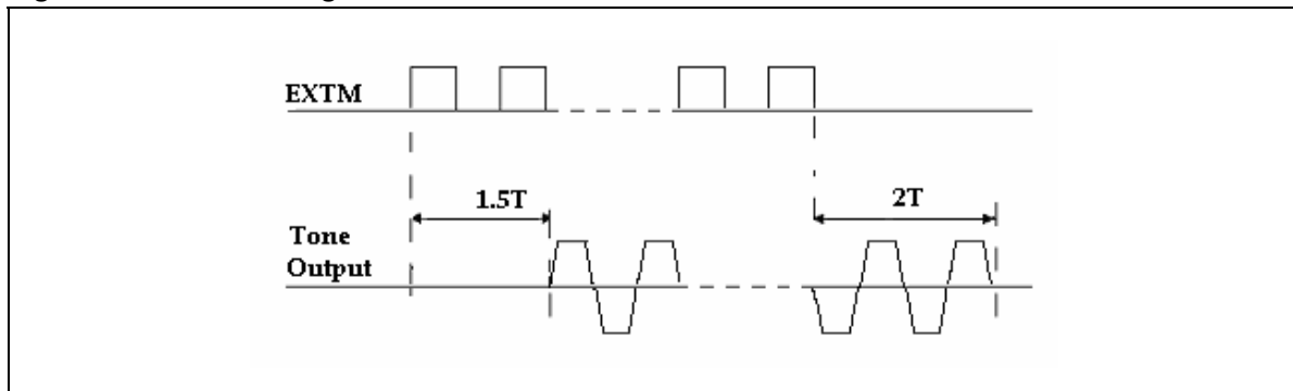
Figure 2. EXTM timings
