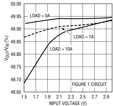
V_{OUT}/V_{IN} Tracking Ratio vs Input Voltage
