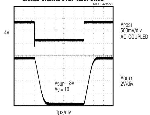
OPERATIONAL AMPLIFIER LARGE-SIGNAL STEP RESPONSE
