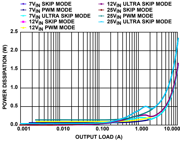
FIGURE 9. V OUT2 = 1.05V POWER DISSIPATION vs LOAD (300kHz)
