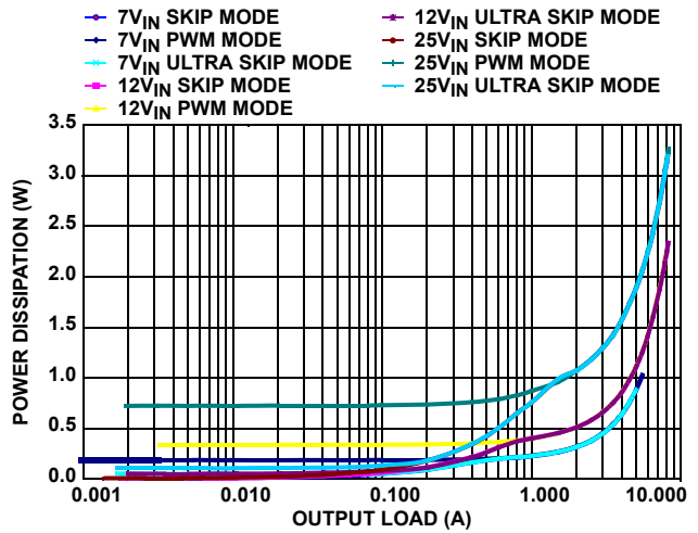
FIGURE 12. V OUT1 = 5V POWER DISSIPATION vs LOAD (400kHz)
