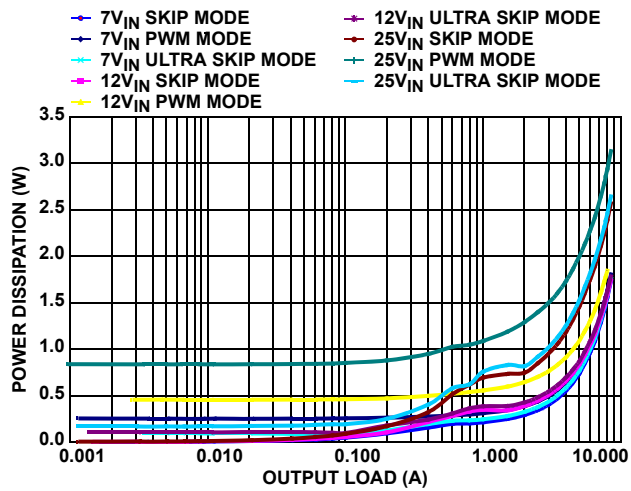
FIGURE 11. V OUT2 = 3.3V POWER DISSIPATION vs LOAD (500kHz)
