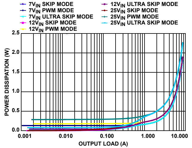
FIGURE 10. V OUT1 = 1.5V POWER DISSIPATION vs LOAD (200kHz)
