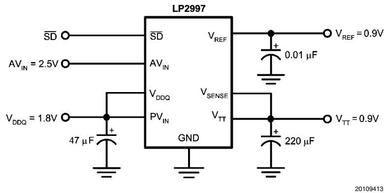
FIGURE 2. Recommended DDR-II Termination
