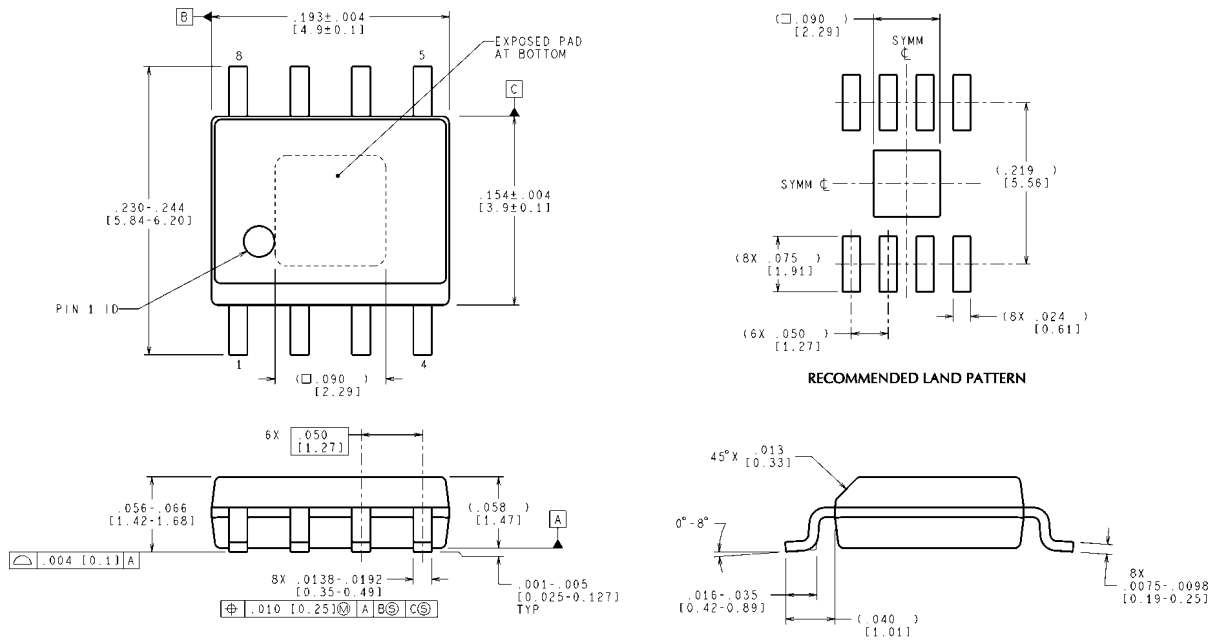
CONTROLLING DIMENSION IS INCH VALUES IN [ ] ARE MILLIMETERS DIMENSIONS IN ( ) FOR REFERENCE ONLY 8-Lead PSOP Package (PSOP-8) NS Package Number MRA08A
