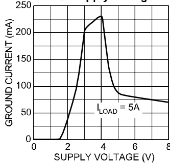
MIC2951x-3.3 Ground Current vs. Supply Voltage
