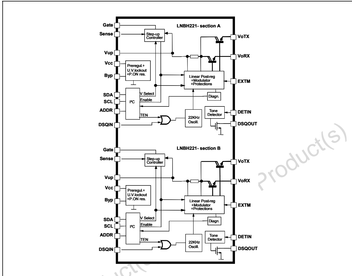
Figure 1. Block diagram
