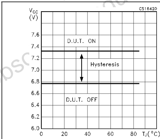
Figure 25. Under voltage lockout threshold vs. temperature
