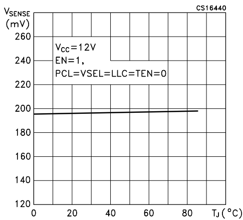
Figure 25 : Current Limit Sense Voltage vs Temperature
