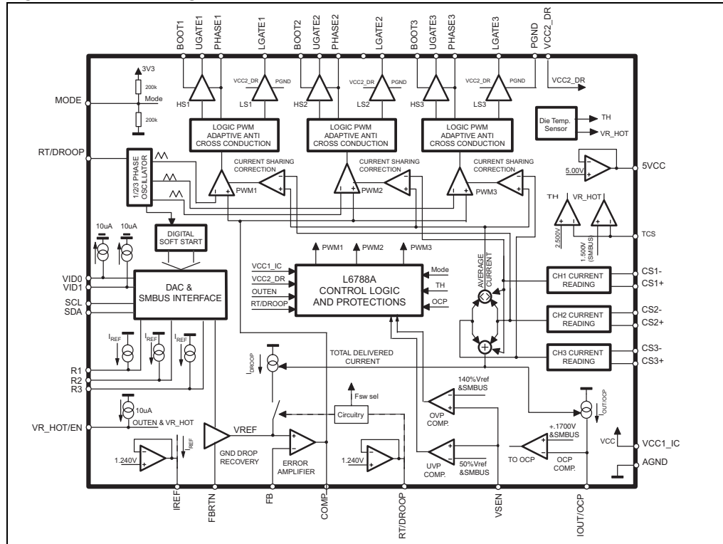
Figure 2. Block diagram
