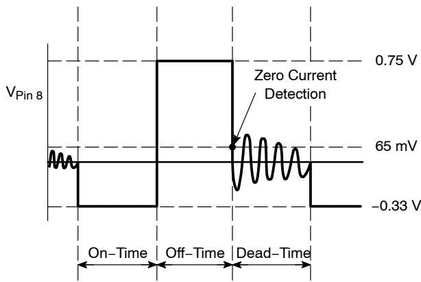
Figure 31. Demagnetization Detection
