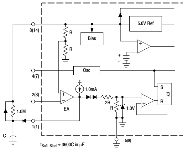
Figure 24. Soft-Start Circuit
